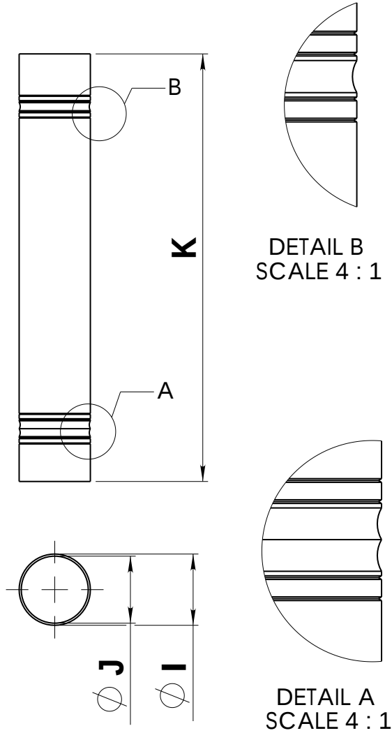
SLIDING PART BOTTOM TUBE
