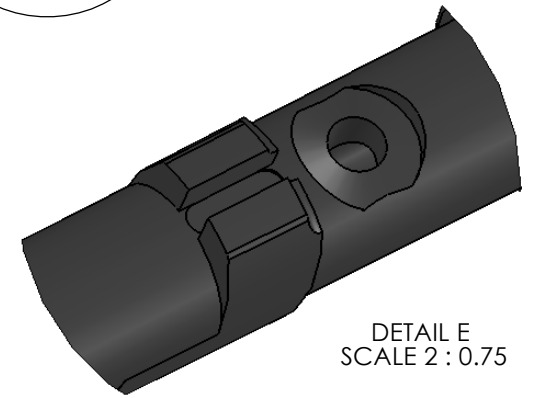
ADDITIONAL VIEWS OF STANDARD 7 KEYED CHANTER
